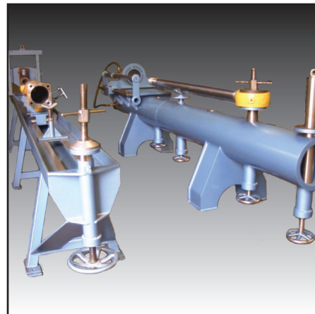
HYDRAULIC CYLINDERS
