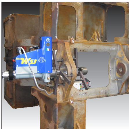
LINE BORING
